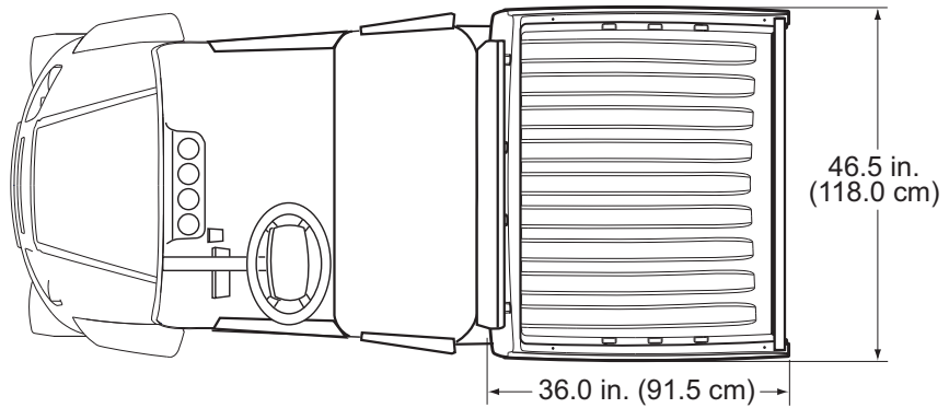
Vehicle Dimensions
