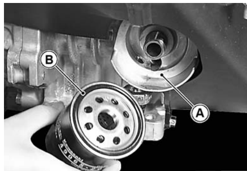
Inspect Oil Filter
