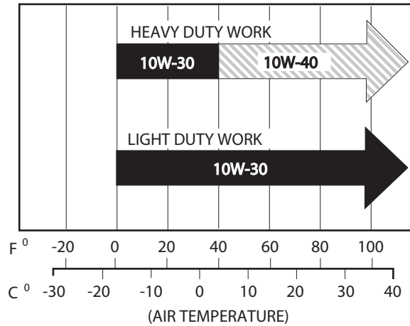
Oil Viscosity Chart
