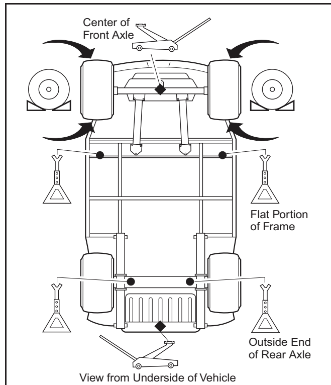
Lifting the Vehicle
