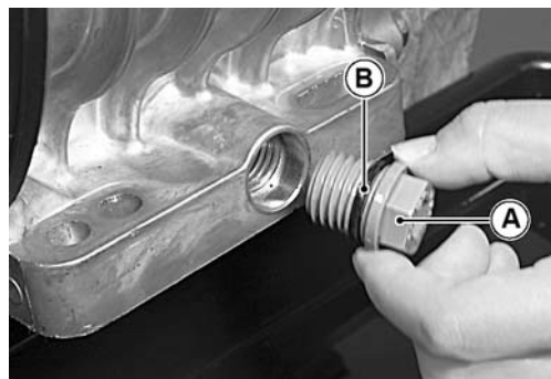
Oil Drain Plug
